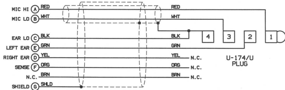
Figure 1: Cable Schematic (41035G-03)
